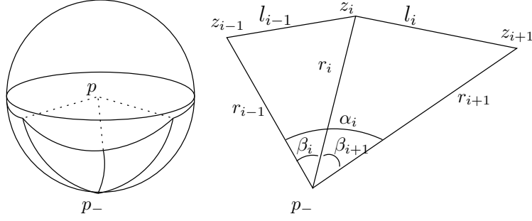
Figure 2: Some notations for the link at p .
