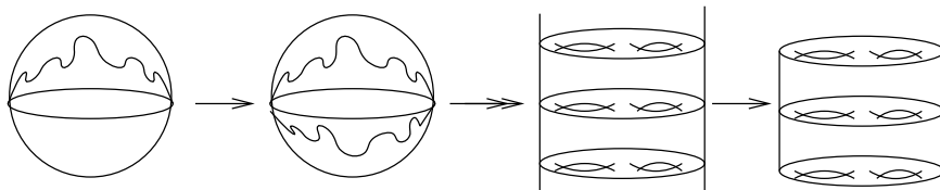
Figure 1: From a Fuchsian polyhedron to a Fuchsian manifold.
